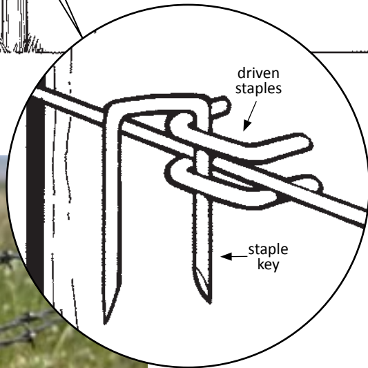
Staple Lock
